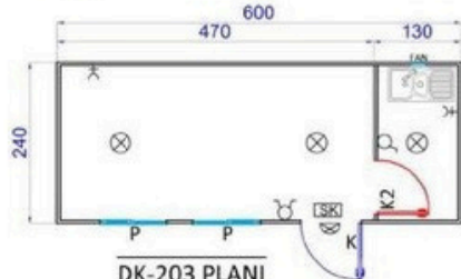
DK-203 PLANI
