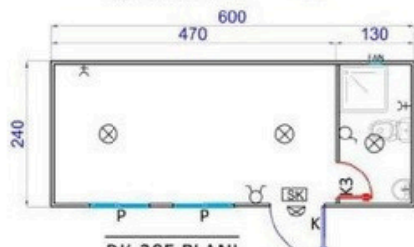
DK-205 PLANI
