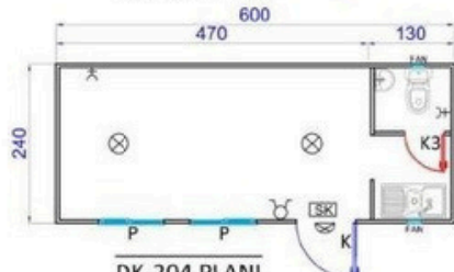
DK-204 PLANI
